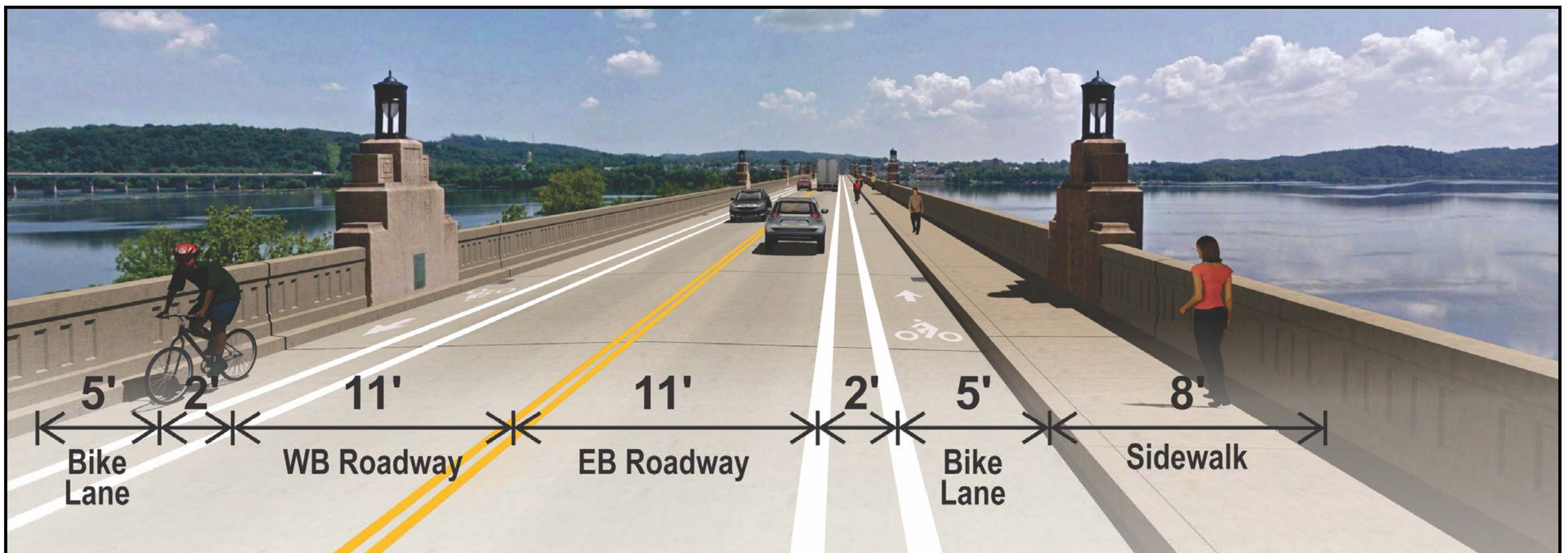
PROPOSED ROADWAY SECTION NEAR WESTERN APPROACH (LOOKING EAST TOWARDS COLUMBIA)
