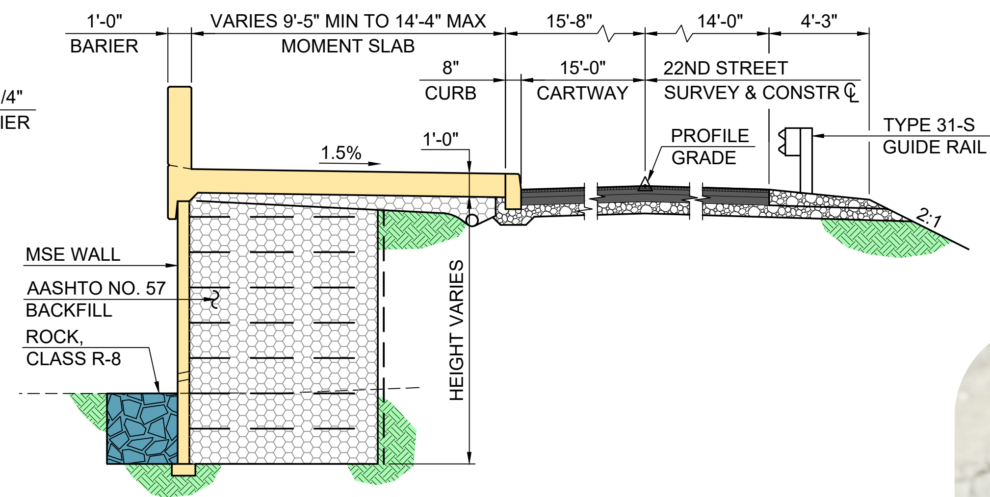
MSE WALL TYPICAL SECTION
