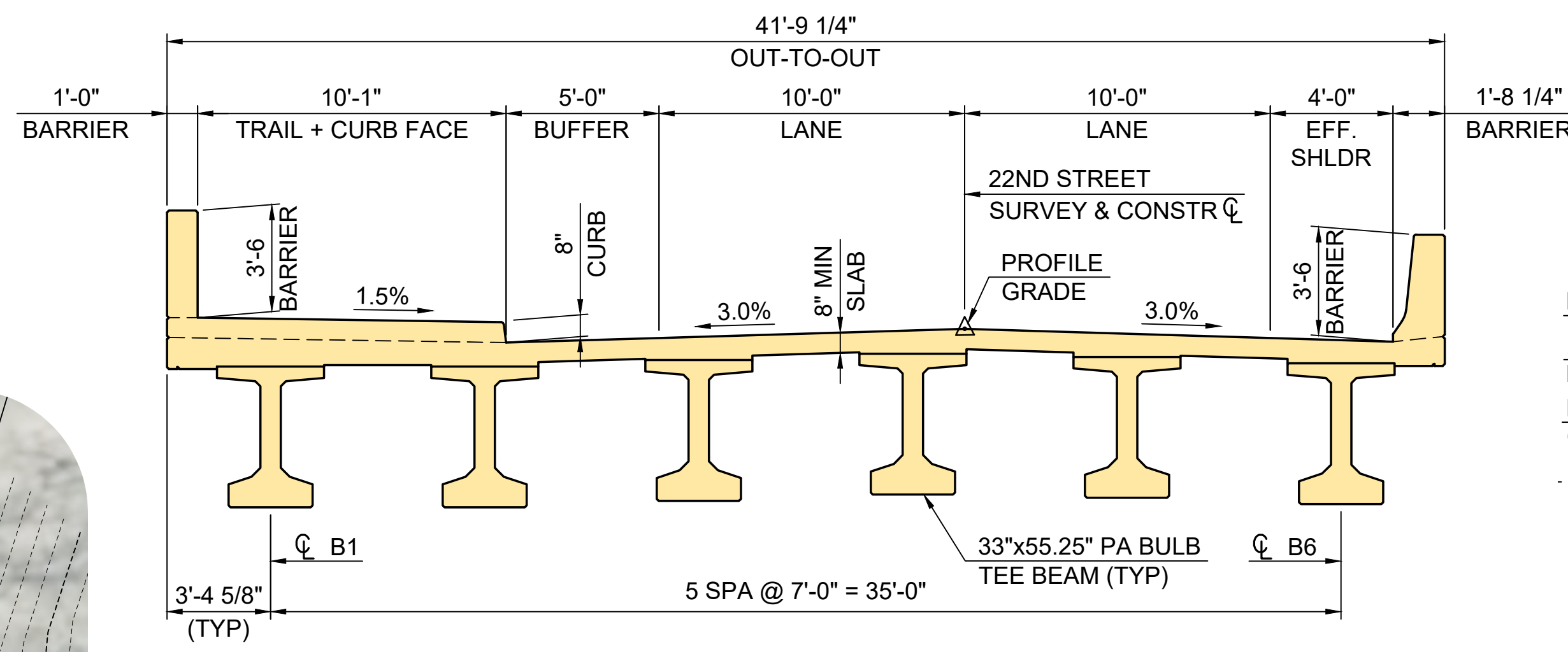
BRIDGE TYPICAL SECTION
