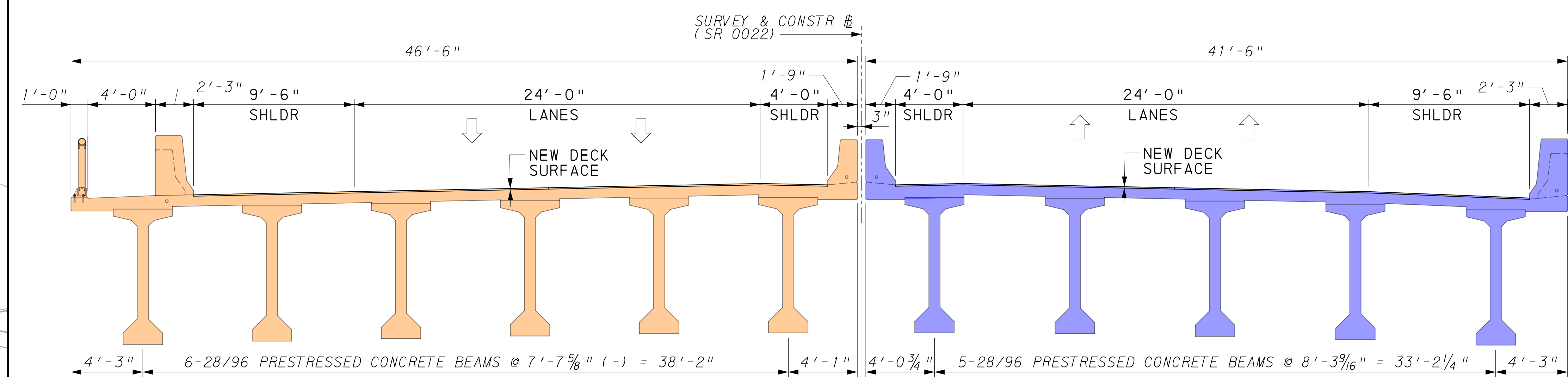
TYPICAL SECTION
