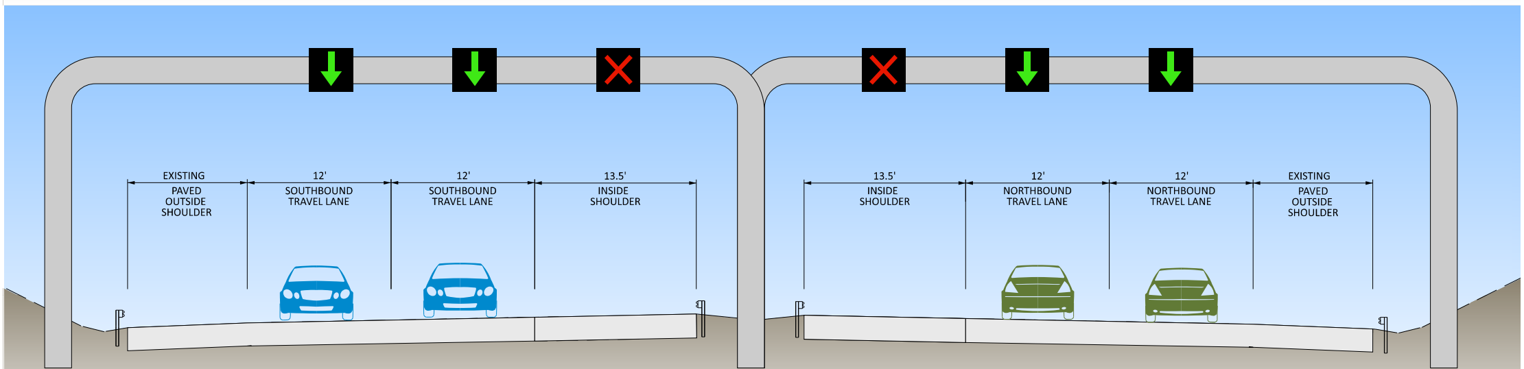
I-476 TYPICAL INACTIVE FLEX LANE
