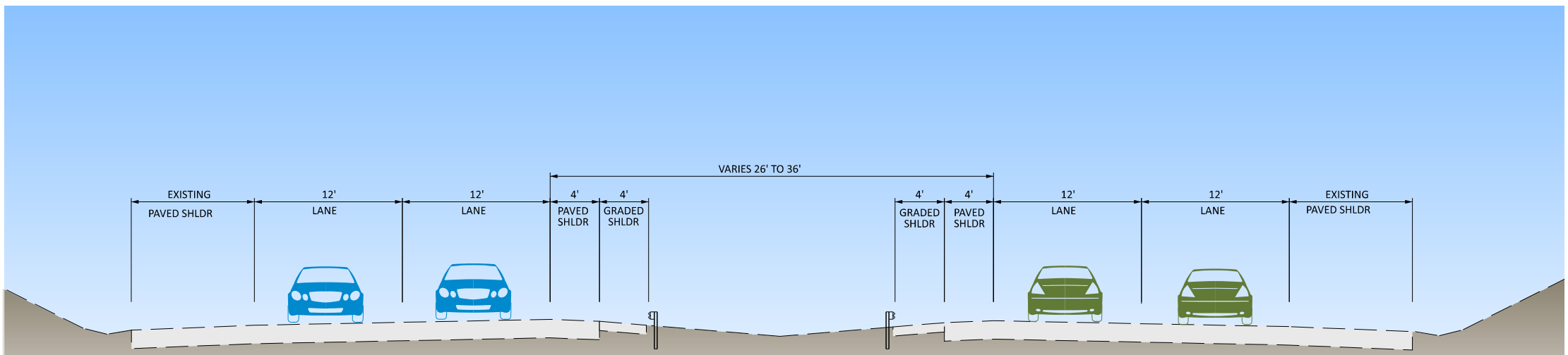
I-476 TYPICAL EXISTING SECTION
