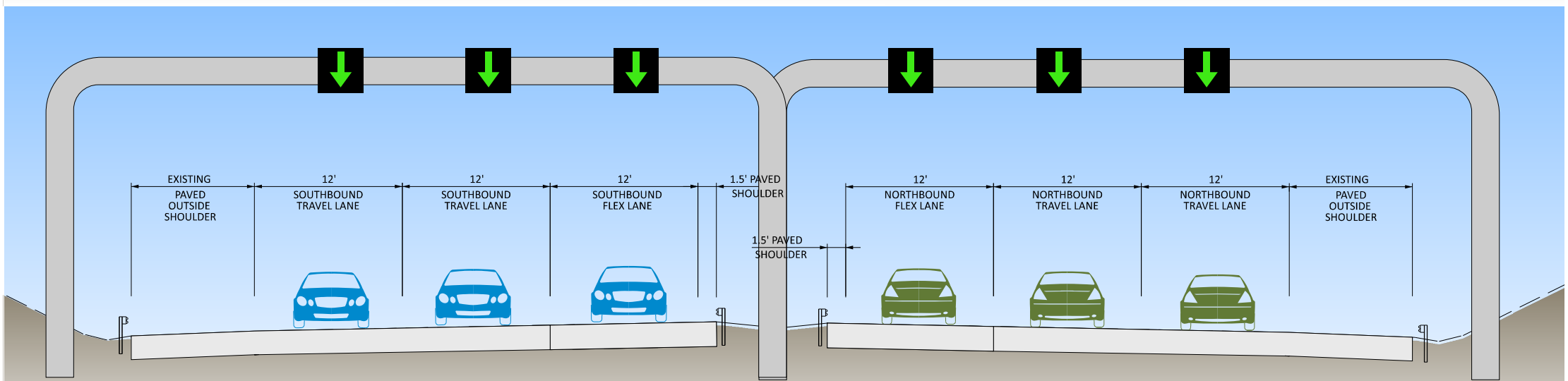
I-476 TYPICAL ACTIVE FLEX LANE
