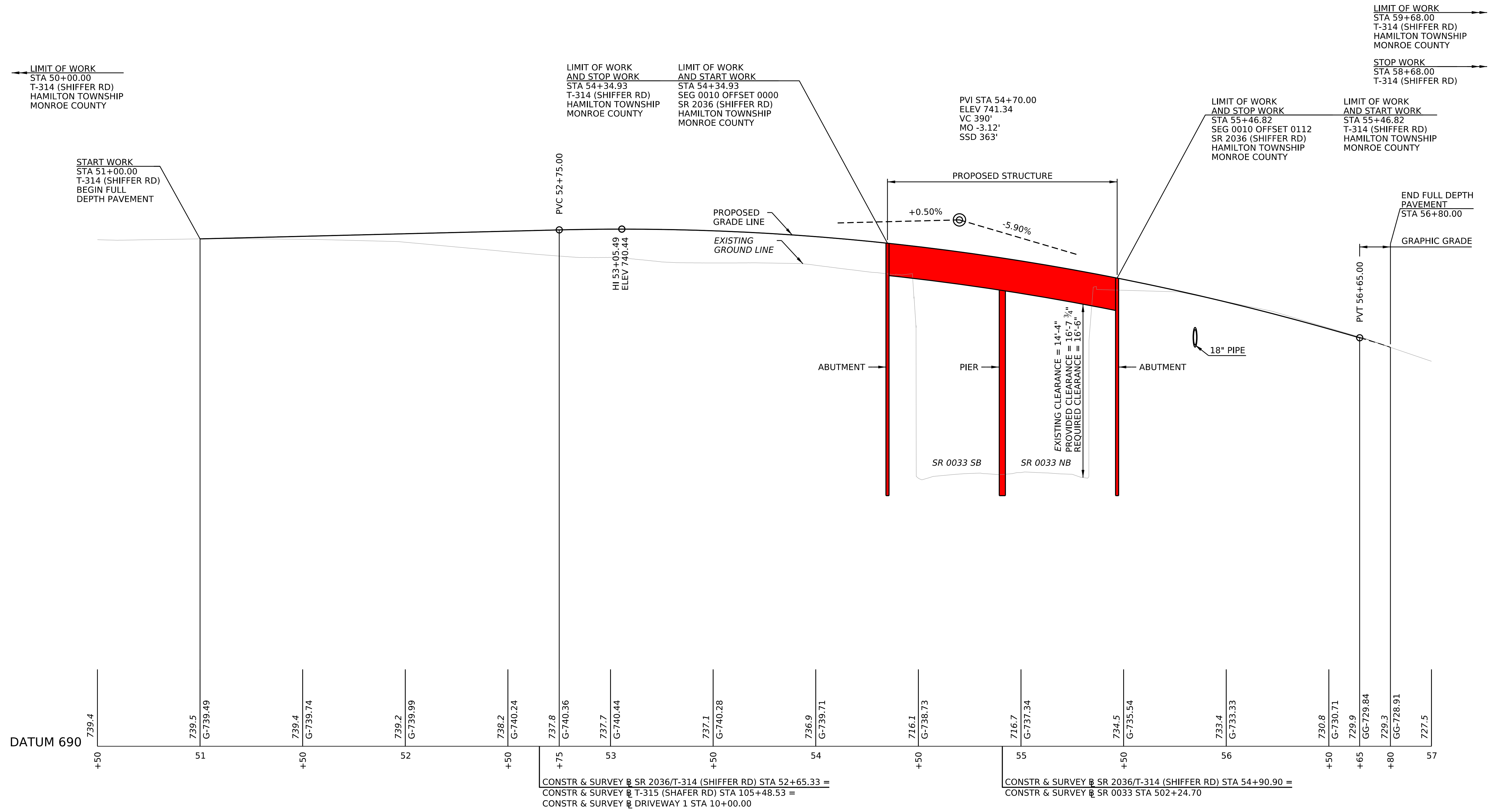
SR 2036/T-314 (SHIFFER RD) - PROFILE
