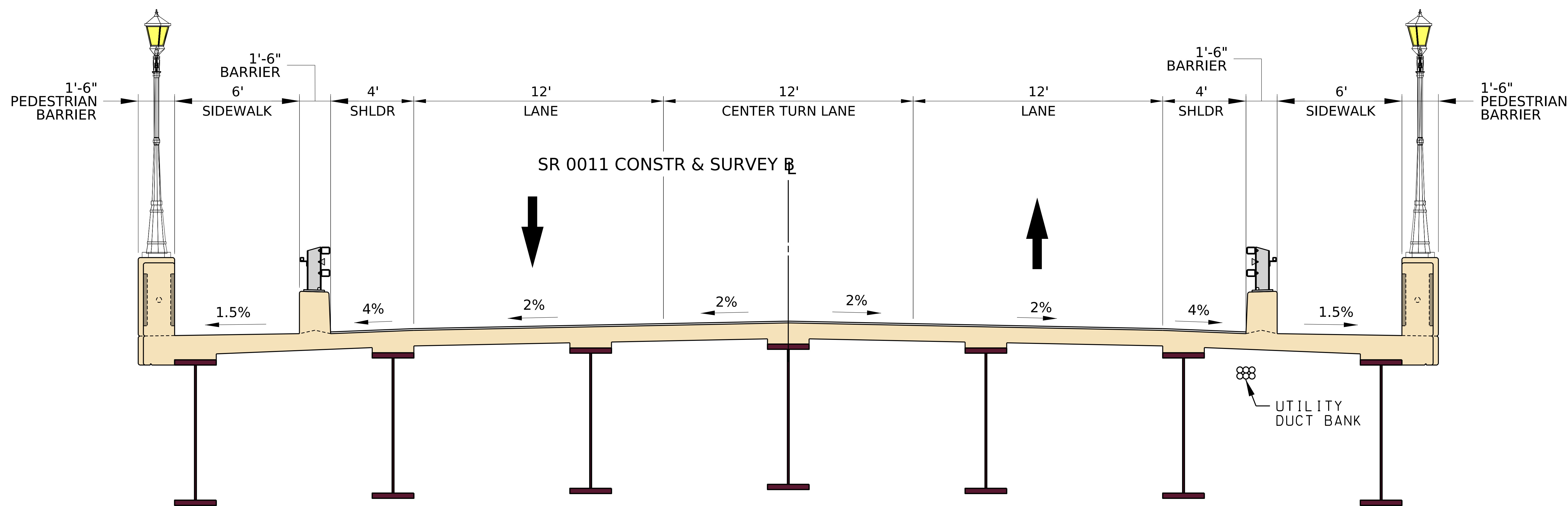
TYPICAL SECTION
