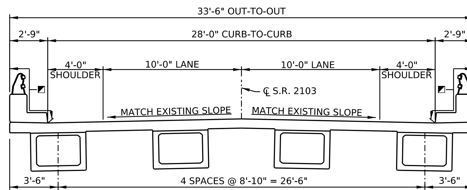
PROPOSED TYPICAL SECTION 2 0 2 4 FEET
